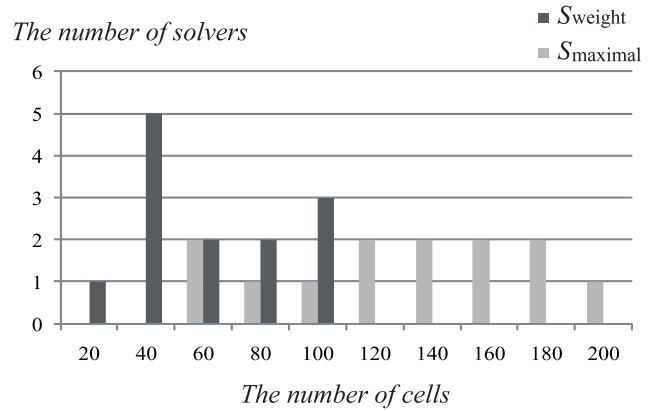
Fig. 11 The distributions of the total numbers of cells to which the solvers in S_{weight} and S_{maximal} gave the correct integers.
