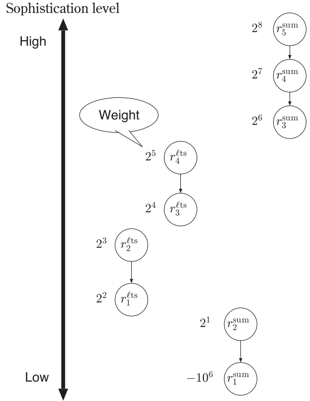
Fig. 9 The generalization relationship among the 9 inference rules and their weights. A directed edge indicates that the inference rule on the starting point is a generalization of the one on the end point.
