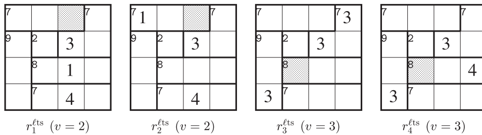
Fig. 7 Situations where the 4 inference rules derived from the Latin square condition are applied. A cell filled with an integer is denoted by (i, j) , and the integer is denoted by v . The cell (i, j) is designated by a shaded square. These conventions are also used in Fig. 8.
