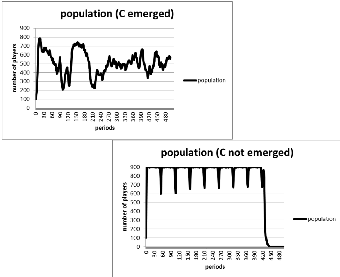
Fig. 3. Two typical examples of simulation. The left is a case (AIIc+AIIID+3ASYM (6), #games=1) in Table 5. The right is a case (AIIc+AIIID+5ASYM (14), #games=5) in Table 6.
